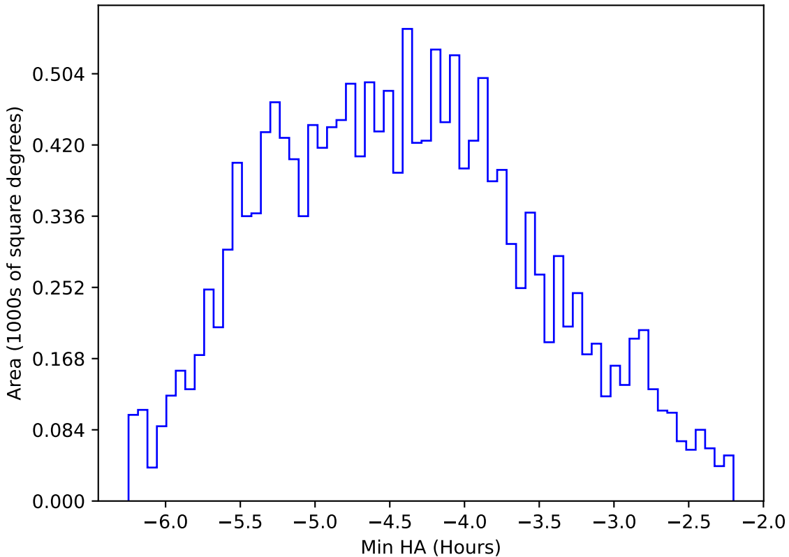
ddf_loaded_half_fl15_v3.4_10yrs WFD r band: Min HA
