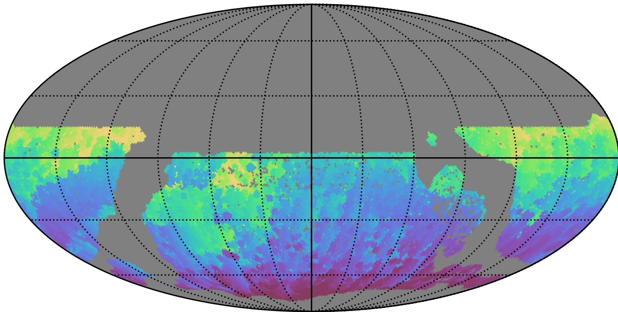
ddf_loaded_half_fl15_v3.4_10yrs WFD i band: Min HA
