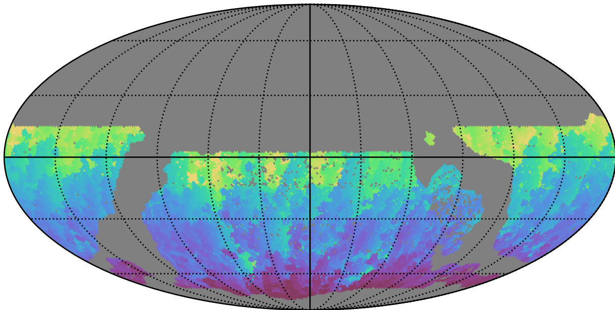
ddf_loaded_half_fl15_v3.4_10yrs WFD g band: Min HA
