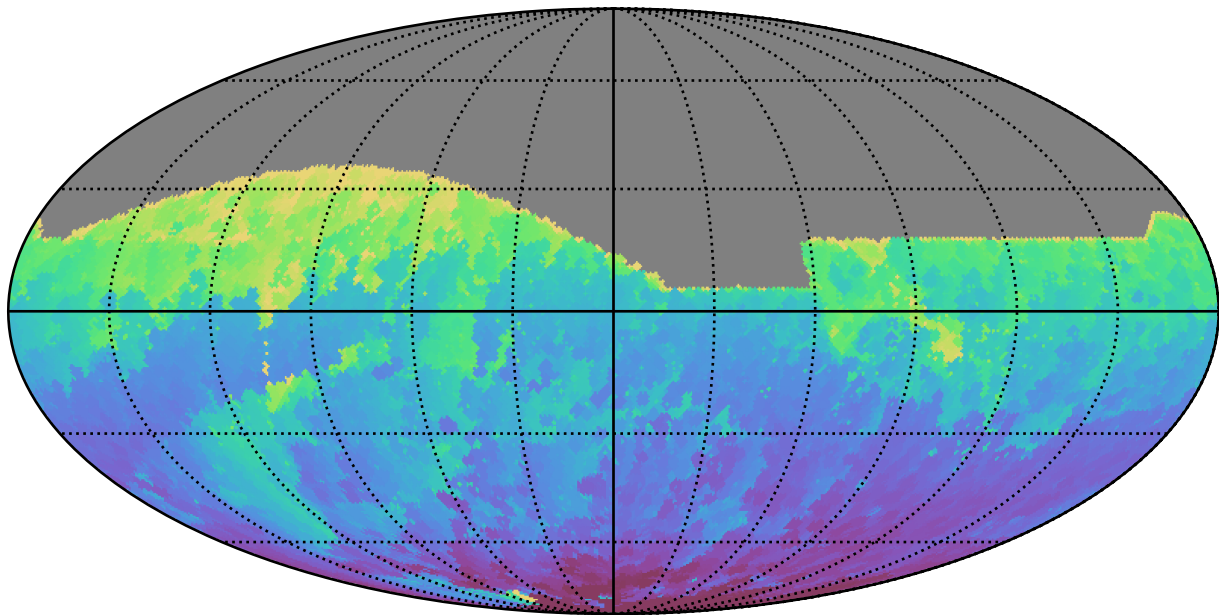
ddf_loaded_half_fl15_v3.4_10yrs All sky z band: Min HA
