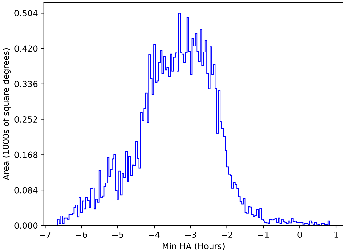
ddf_loaded_half_fl15_v3.4_10yrs All sky y band: Min HA
