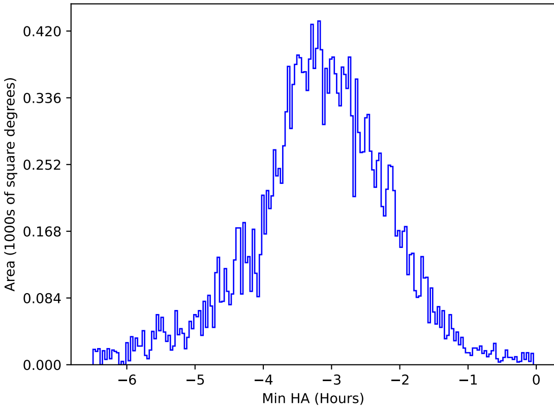
ddf_loaded_half_fl15_v3.4_10yrs All sky u band: Min HA
