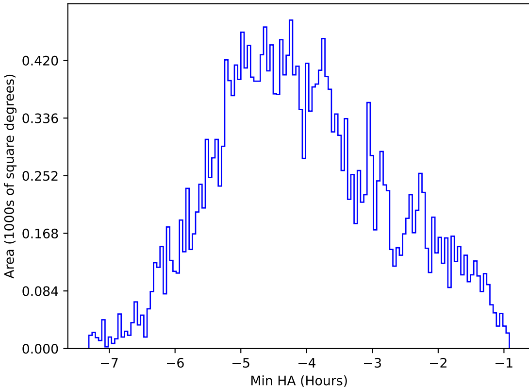
ddf_loaded_half_fl15_v3.4_10yrs All sky i band: Min HA
