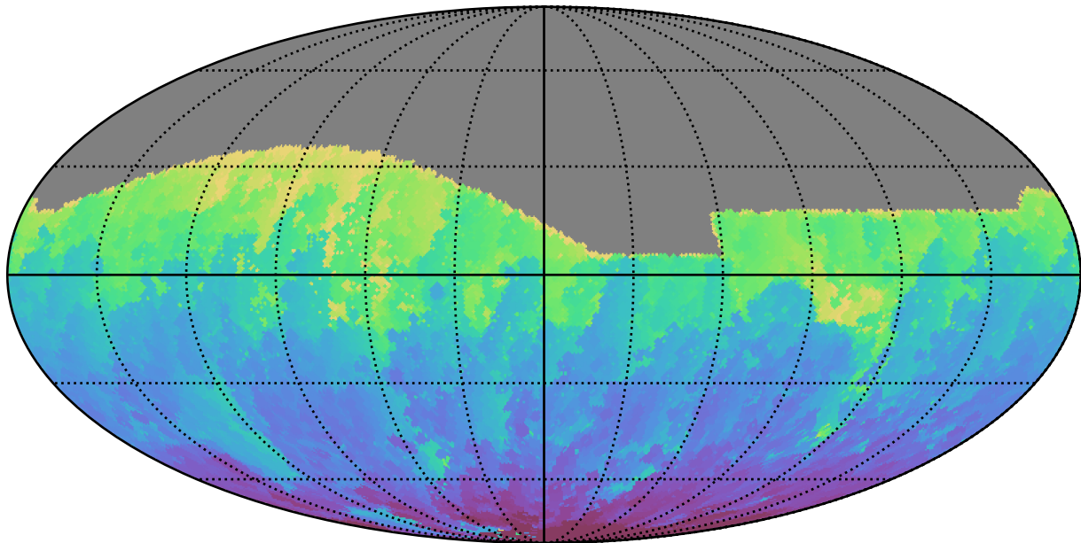
ddf_loaded_half_fl15_v3.4_10yrs All sky g band: Min HA
