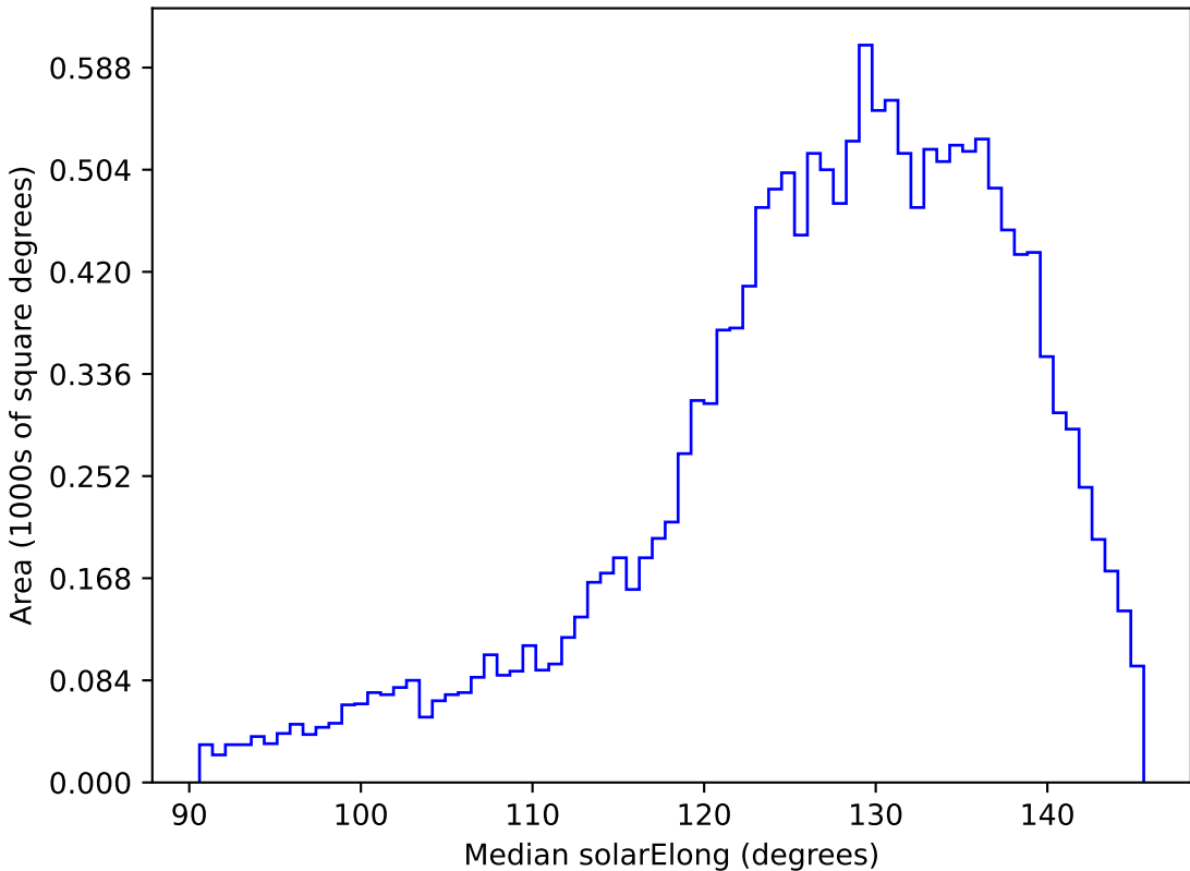
ddf_loaded_half_fl15_v3.4_10yrs WFD z band: Median solarElong
