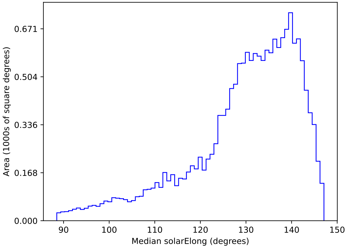
ddf_loaded_half_fl15_v3.4_10yrs WFD y band: Median solarElong
