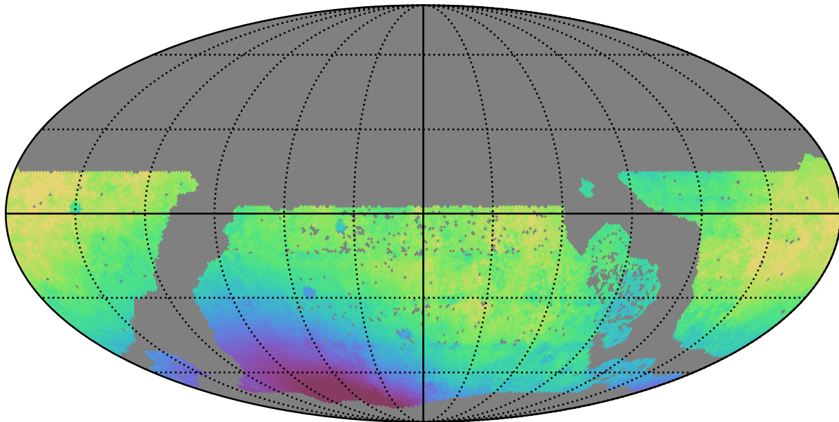
ddf_loaded_half_fl15_v3.4_10yrs WFD r band: Median solarElong
