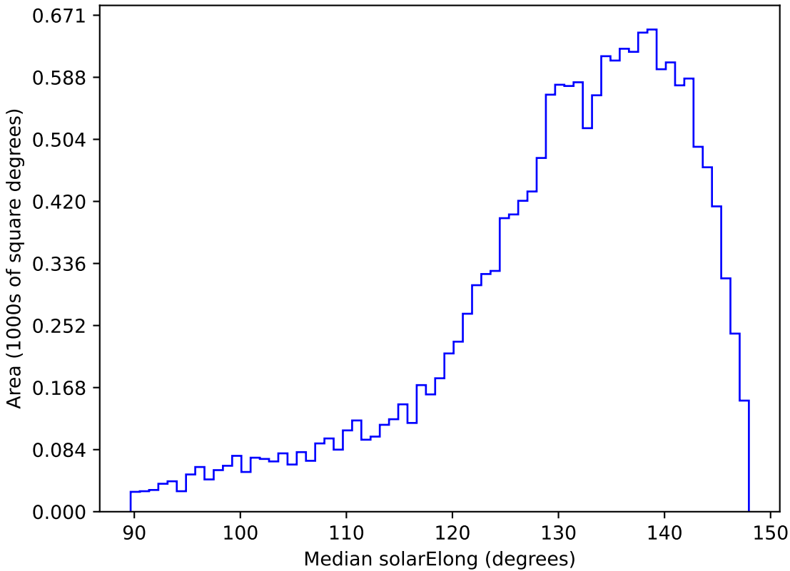
ddf_loaded_half_fl15_v3.4_10yrs WFD r band: Median solarElong
