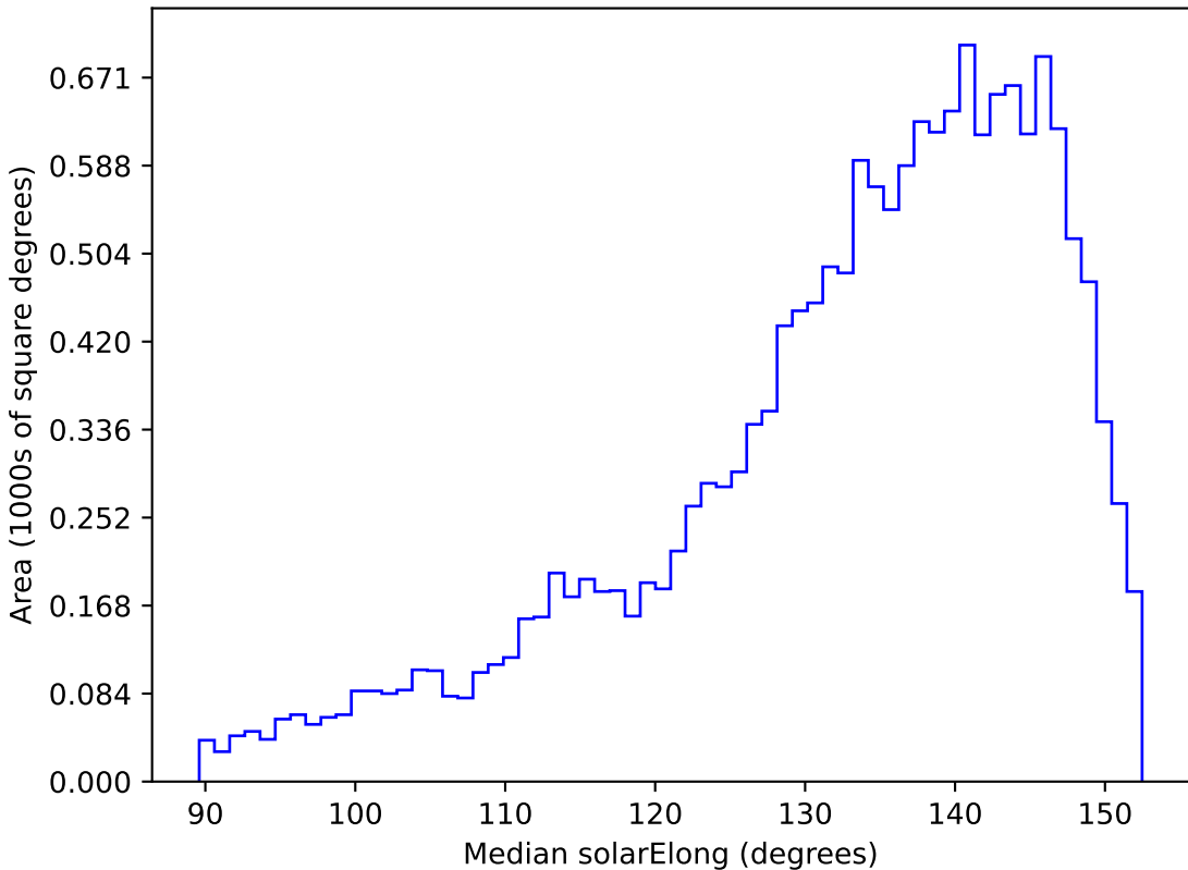
ddf_loaded_half_fl15_v3.4_10yrs WFD g band: Median solarElong
