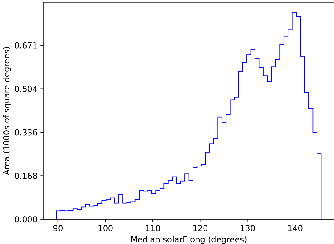
ddf_loaded_half_fl15_v3.4_10yrs WFD all bands: Median solarElong
