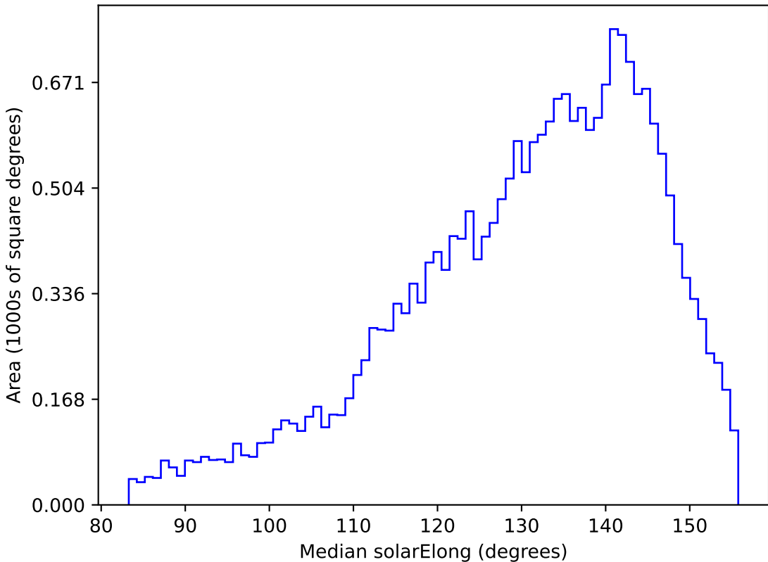
ddf_loaded_half_fl15_v3.4_10yrs All sky u band: Median solarElong
