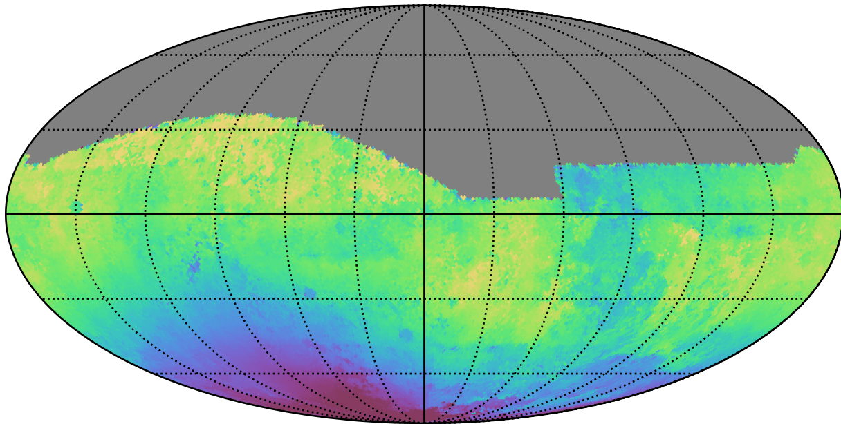
ddf_loaded_half_fl15_v3.4_10yrs All sky g band: Median solarElong
