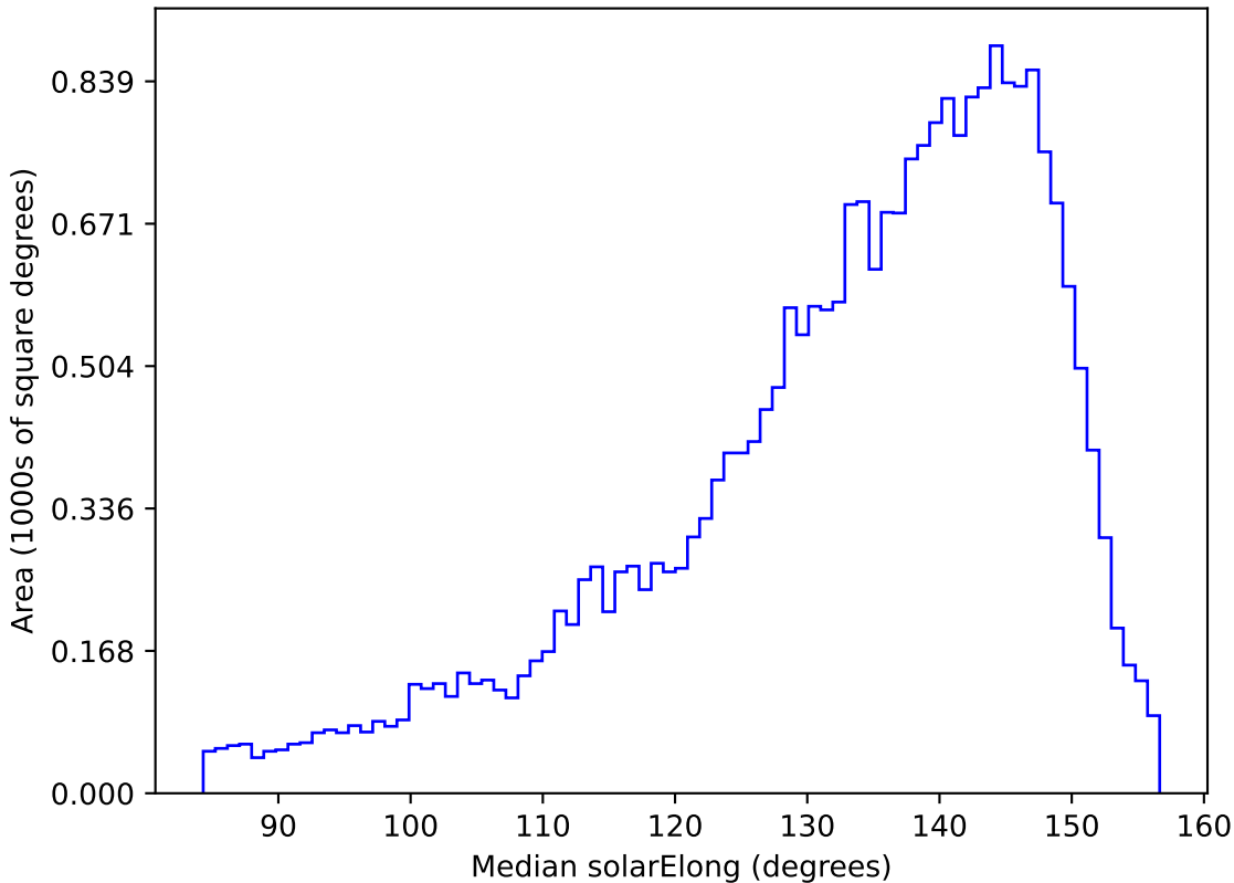
ddf_loaded_half_fl15_v3.4_10yrs All sky g band: Median solarElong
