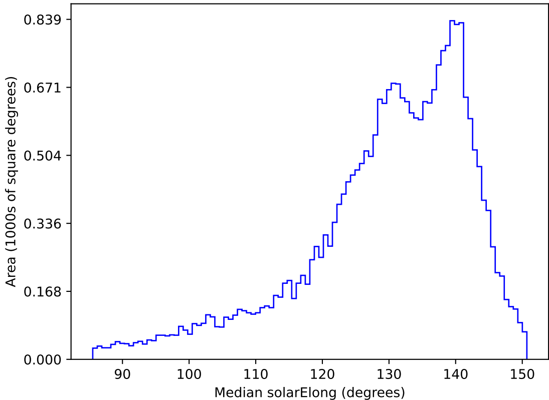
ddf_loaded_half_fl15_v3.4_10yrs All sky all bands: Median solarElong
