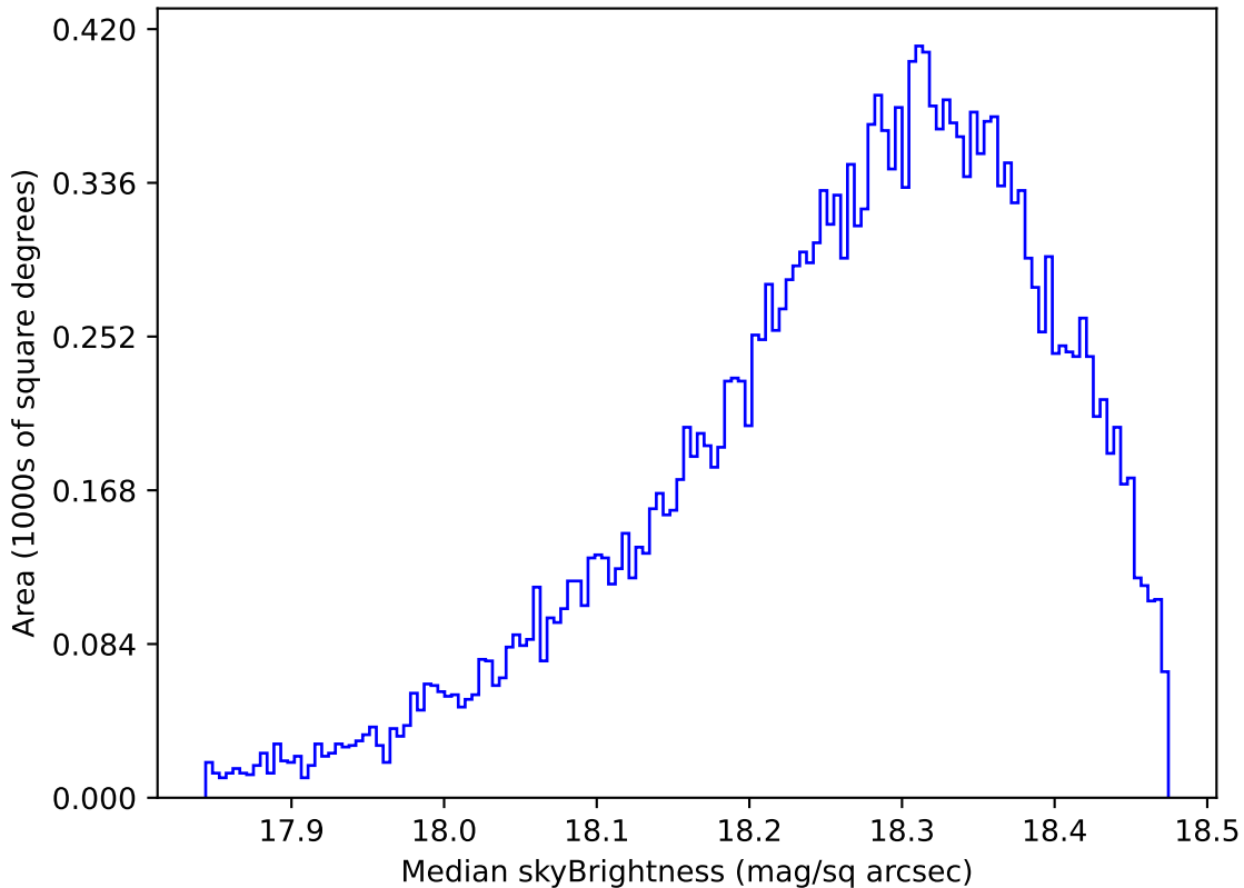
ddf_loaded_half_fl15_v3.4_10yrs Yr 1 y band: Median skyBrightness
