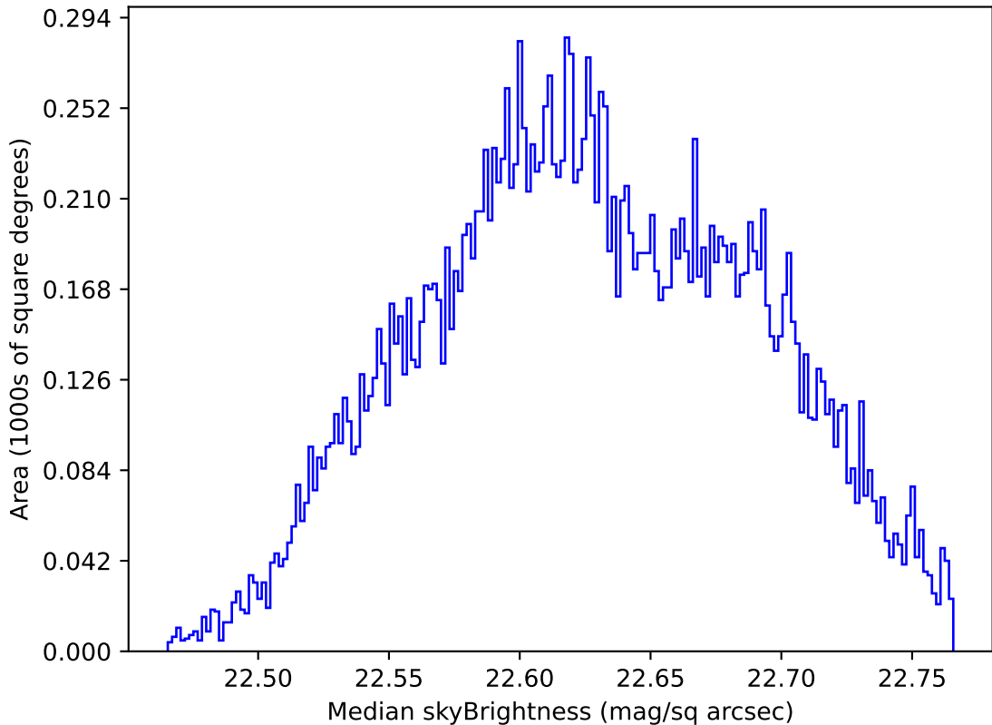
ddf_loaded_half_fl15_v3.4_10yrs Yr 1 u band: Median skyBrightness
