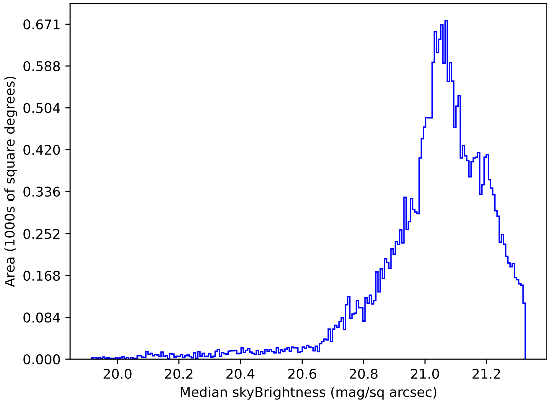
ddf_loaded_half_fl15_v3.4_10yrs Yr 1 r band: Median skyBrightness
