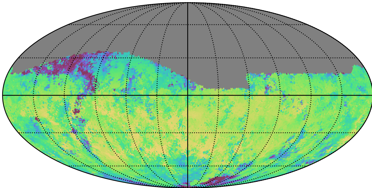
ddf_loaded_half_fl15_v3.4_10yrs Yr 1 i band: Median skyBrightness
