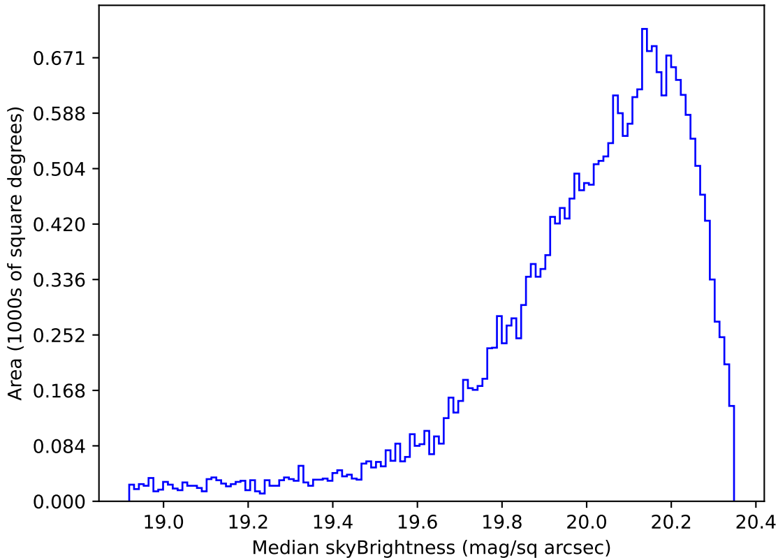
ddf_loaded_half_fl15_v3.4_10yrs Yr 1 i band: Median skyBrightness
