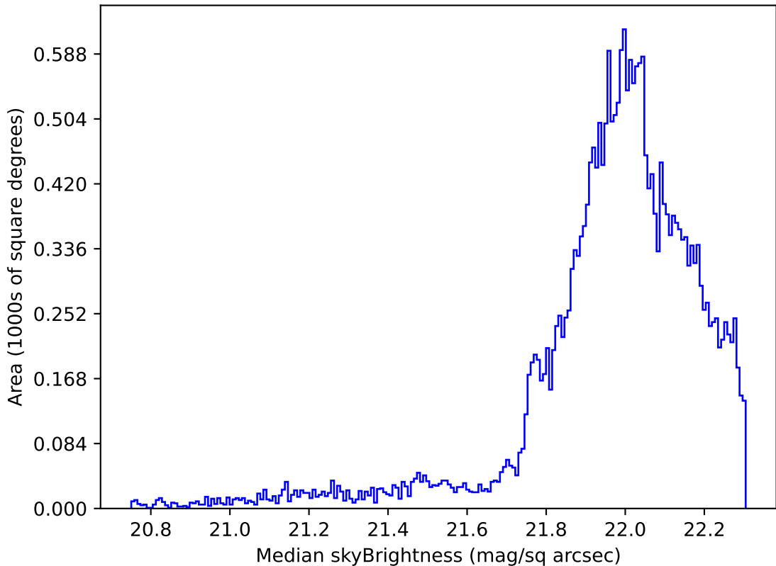
ddf_loaded_half_fl15_v3.4_10yrs Yr 1 g band: Median skyBrightness
