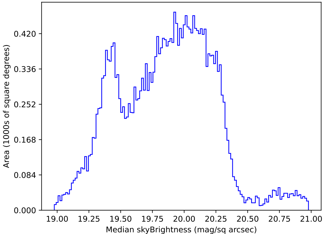
ddf_loaded_half_fl15_v3.4_10yrs Yr 1 all bands: Median skyBrightness
