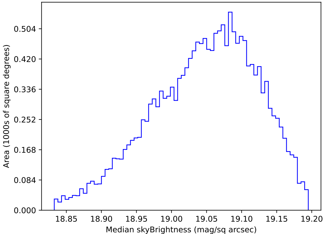
ddf_loaded_half_fl15_v3.4_10yrs WFD z band: Median skyBrightness
