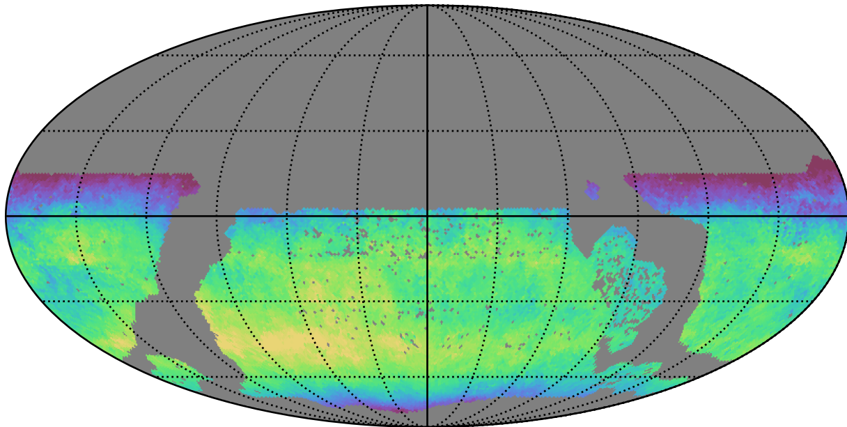
ddf_loaded_half_fl15_v3.4_10yrs WFD y band: Median skyBrightness
