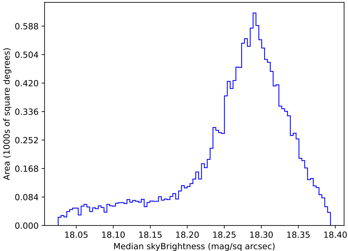
ddf_loaded_half_fl15_v3.4_10yrs WFD y band: Median skyBrightness
