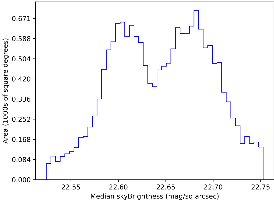
ddf_loaded_half_fl15_v3.4_10yrs WFD u band: Median skyBrightness
