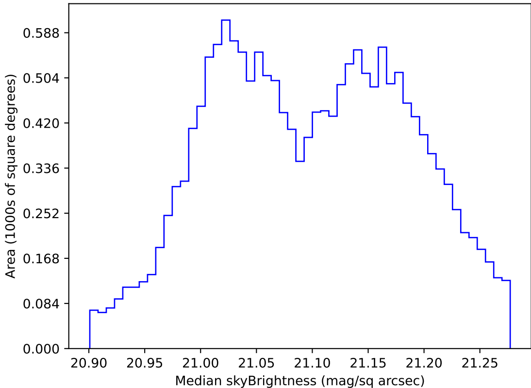
ddf_loaded_half_fl15_v3.4_10yrs WFD r band: Median skyBrightness
