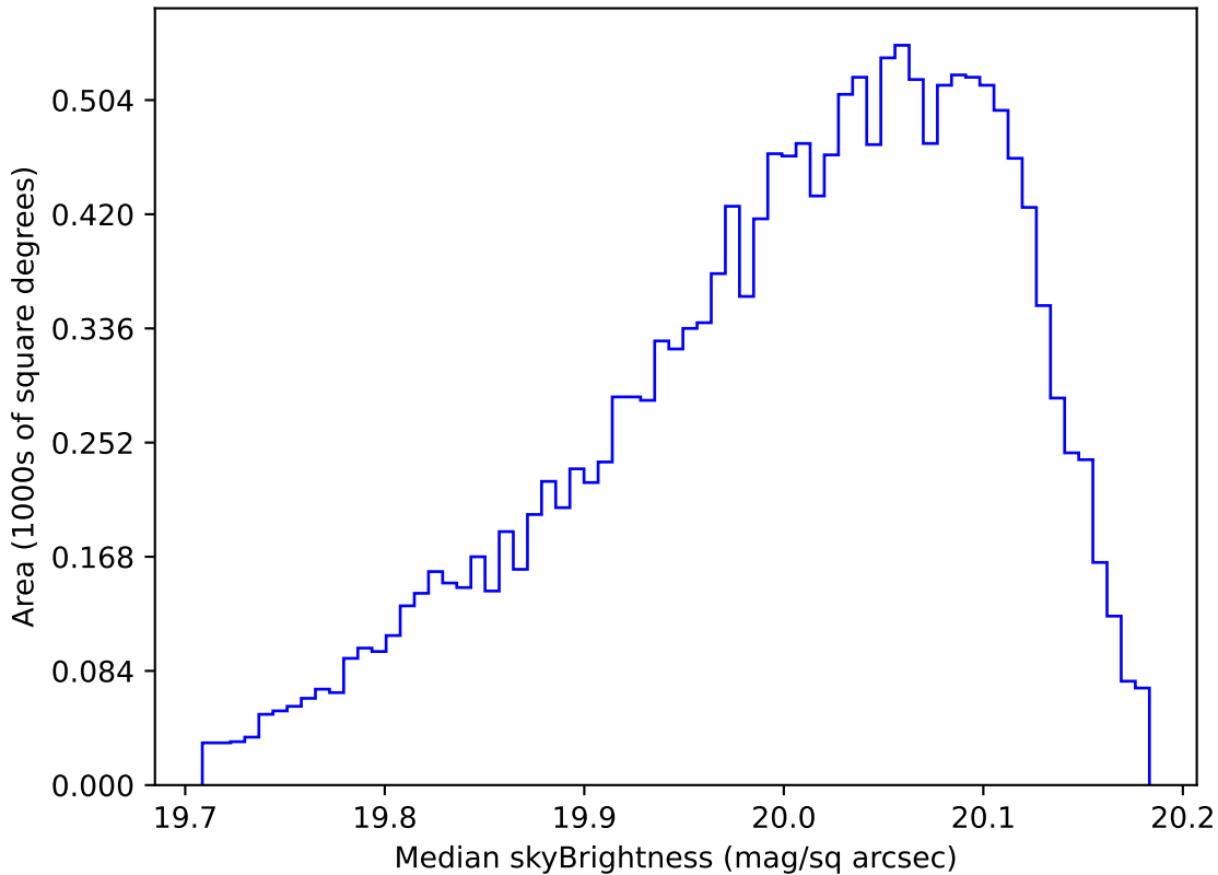
ddf_loaded_half_fl15_v3.4_10yrs WFD i band: Median skyBrightness
