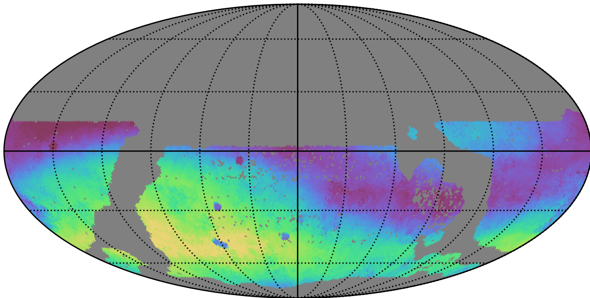
ddf_loaded_half_fl15_v3.4_10yrs WFD g band: Median skyBrightness
