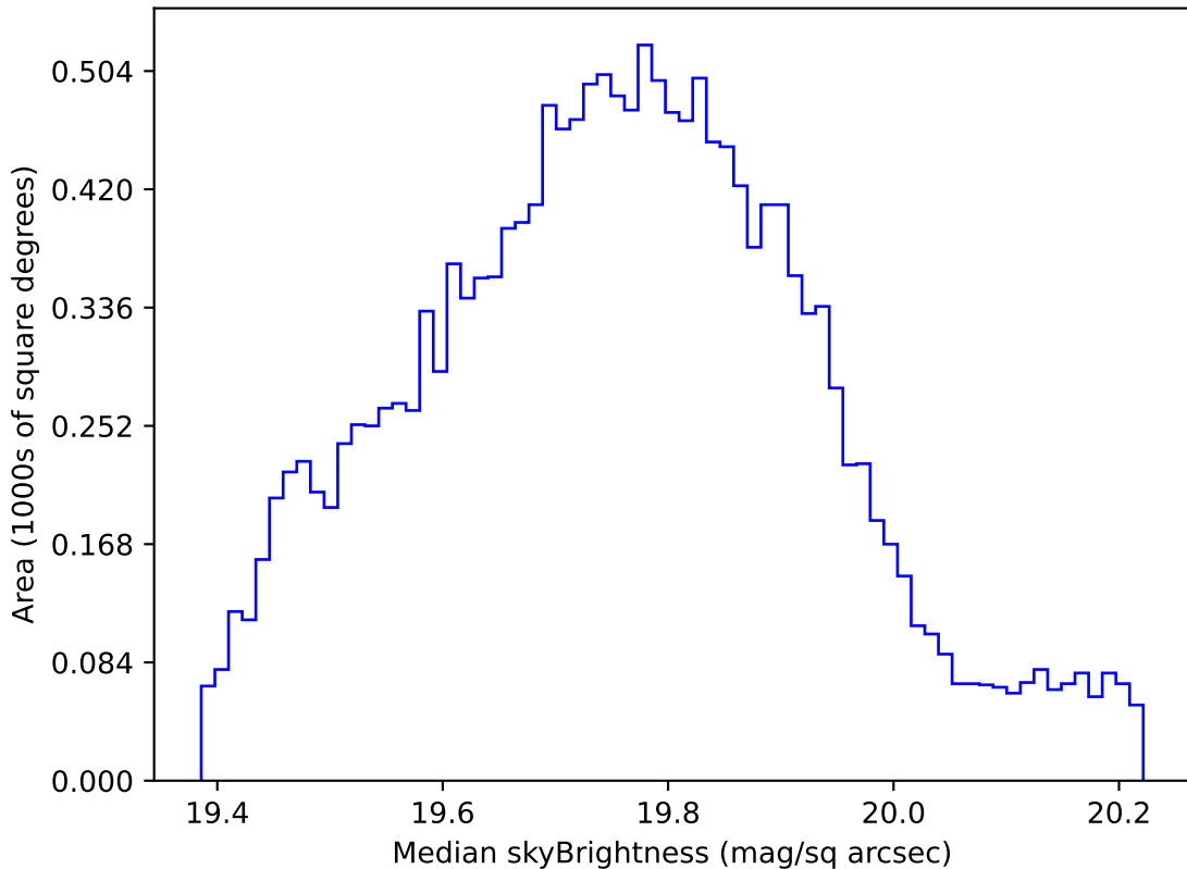
ddf_loaded_half_fl15_v3.4_10yrs WFD all bands: Median skyBrightness
