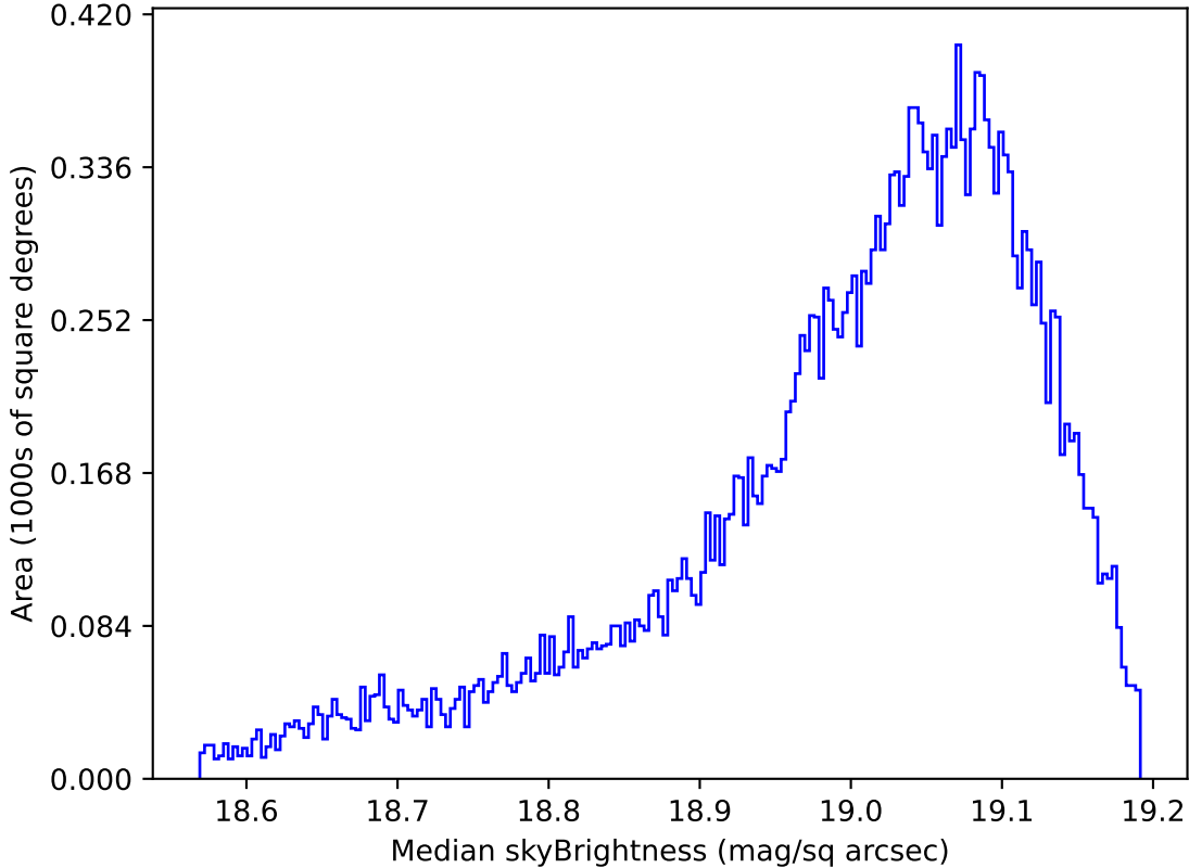
ddf_loaded_half_fl15_v3.4_10yrs All sky z band: Median skyBrightness
