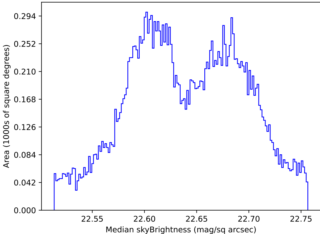
ddf_loaded_half_fl15_v3.4_10yrs All sky u band: Median skyBrightness
