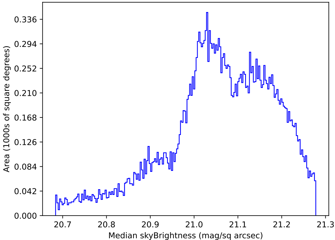
ddf_loaded_half_fl15_v3.4_10yrs All sky r band: Median skyBrightness
