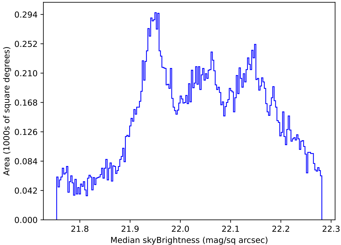
ddf_loaded_half_fl15_v3.4_10yrs All sky g band: Median skyBrightness
