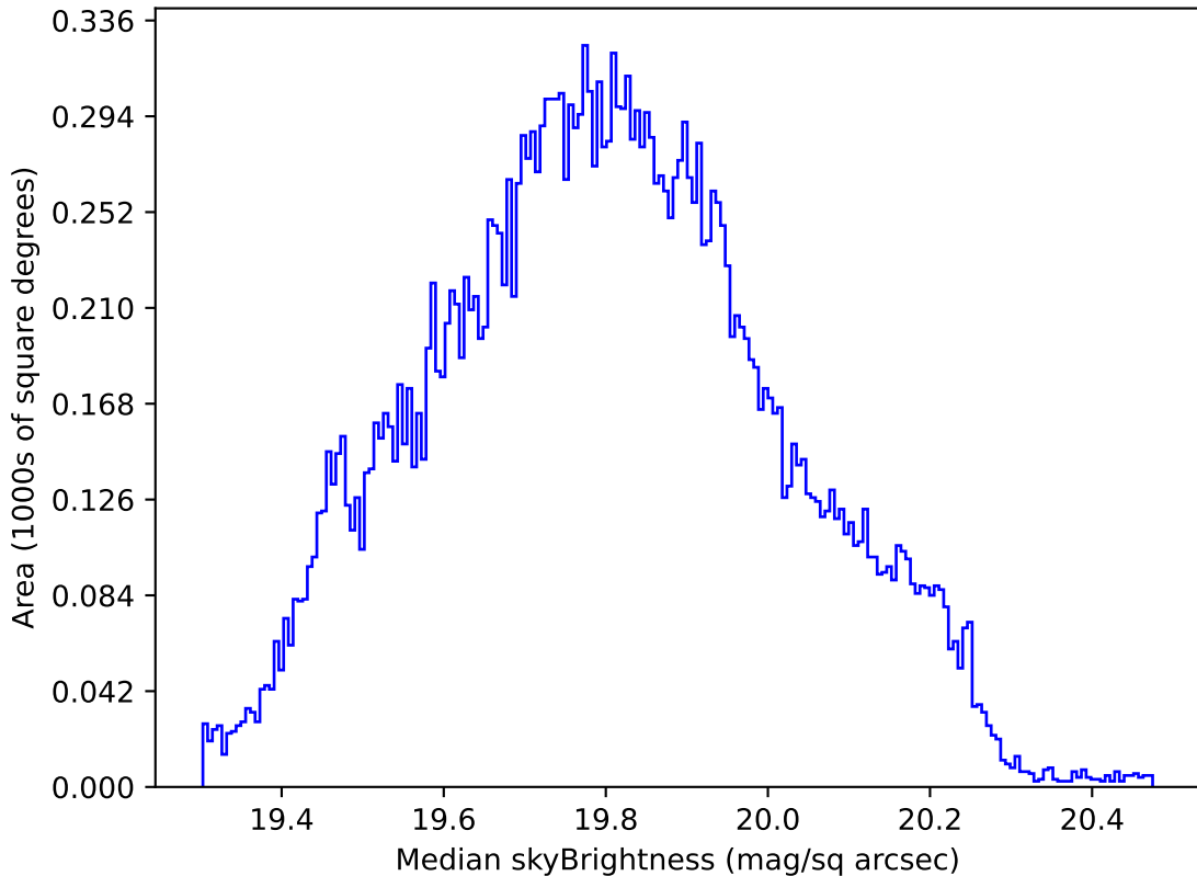
ddf_loaded_half_fl15_v3.4_10yrs All sky all bands: Median skyBrightness
