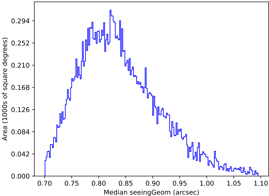
ddf_loaded_half_fl15_v3.4_10yrs Yr 1 y band: Median seeingGeom
