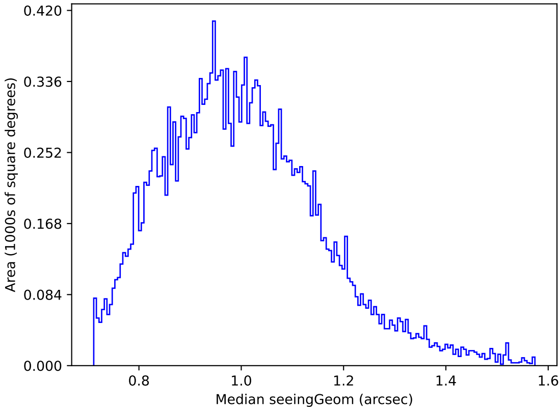
ddf_loaded_half_fl15_v3.4_10yrs Yr 1 u band: Median seeingGeom
