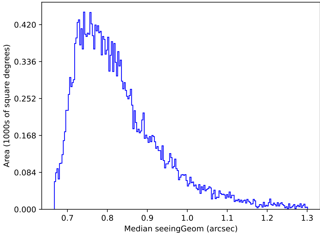
ddf_loaded_half_fl15_v3.4_10yrs Yr 1 i band: Median seeingGeom
