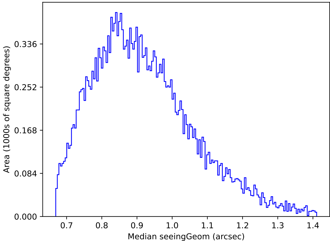
ddf_loaded_half_fl15_v3.4_10yrs Yr 1 g band: Median seeingGeom
