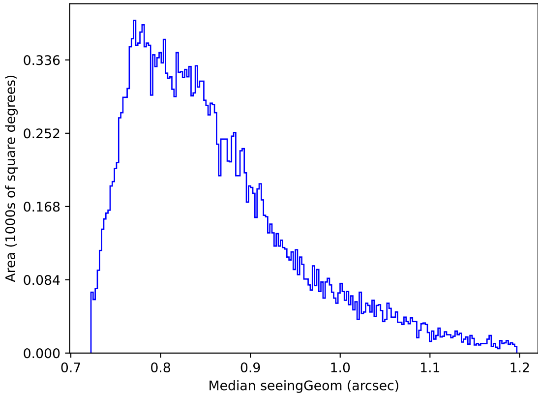
ddf_loaded_half_fl15_v3.4_10yrs Yr 1 all bands: Median seeingGeom
