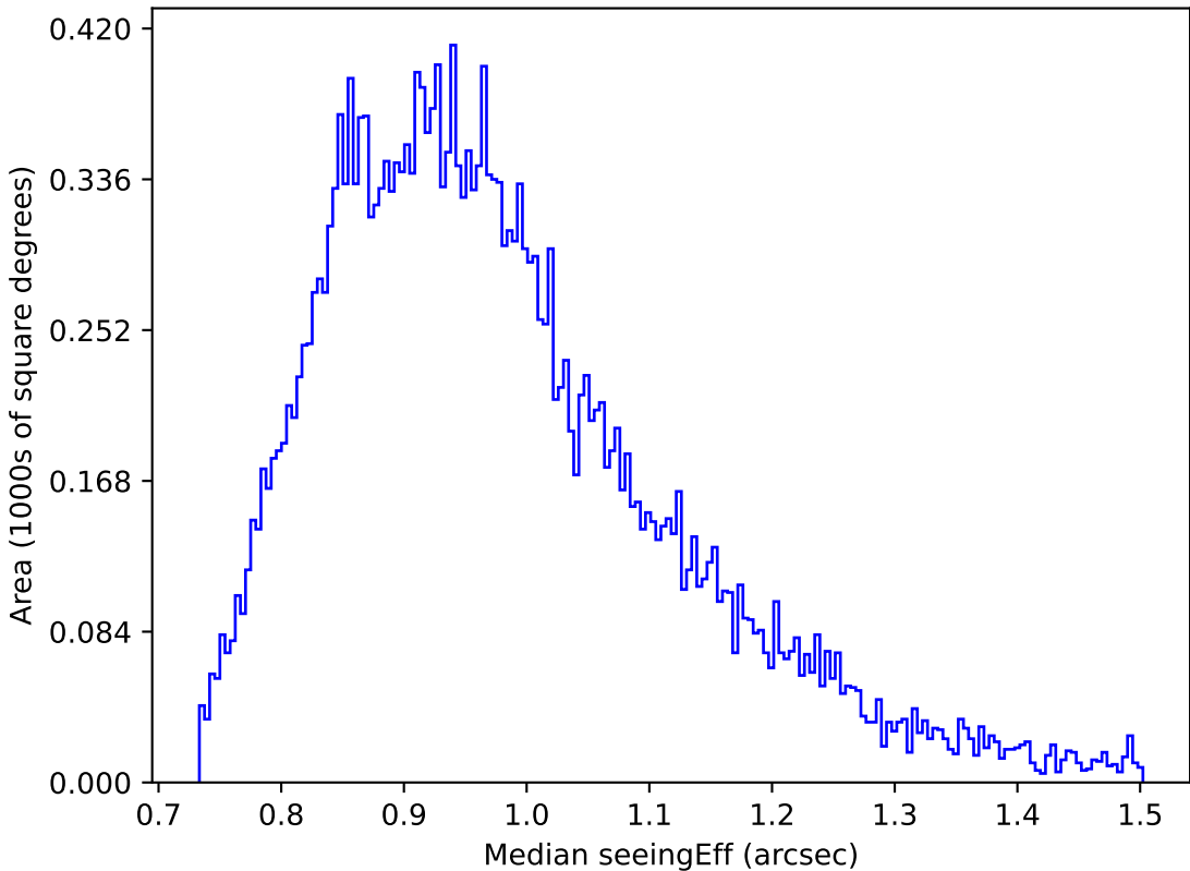
ddf_loaded_half_fl15_v3.4_10yrs Yr 1 z band: Median seeingEff
