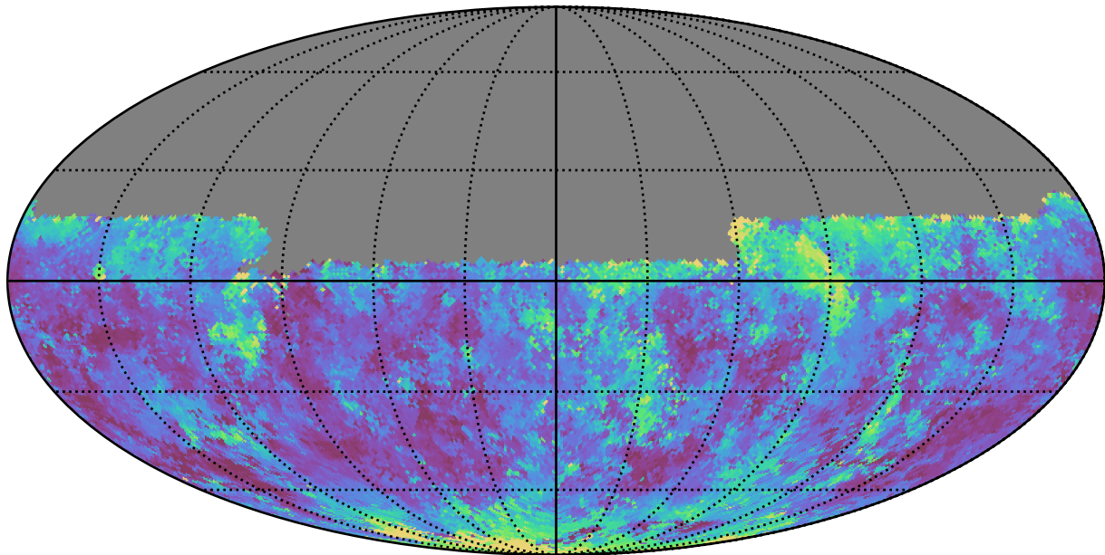
ddf_loaded_half_fl15_v3.4_10yrs Yr 1 y band: Median seeingEff
