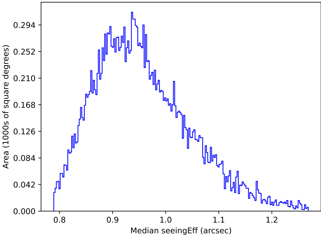
ddf_loaded_half_fl15_v3.4_10yrs Yr 1 y band: Median seeingEff
