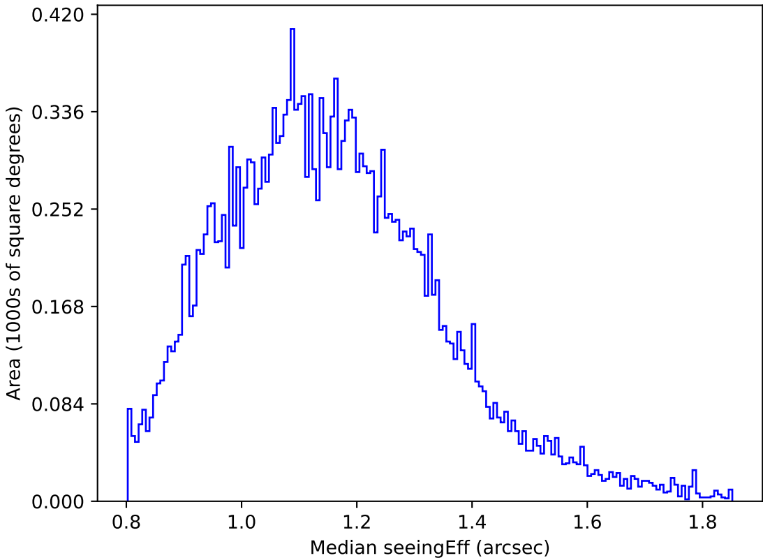
ddf_loaded_half_fl15_v3.4_10yrs Yr 1 u band: Median seeingEff
