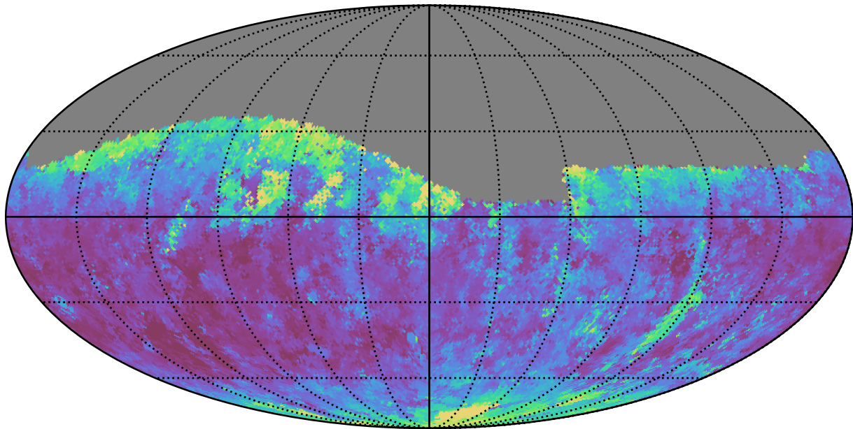
ddf_loaded_half_fl15_v3.4_10yrs Yr 1 r band: Median seeingEff
