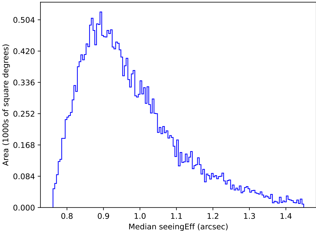
ddf_loaded_half_fl15_v3.4_10yrs Yr 1 r band: Median seeingEff
