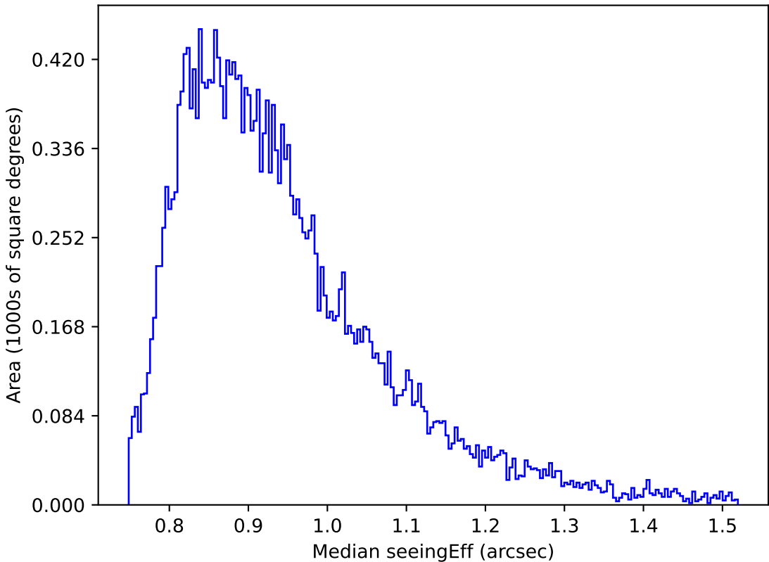
ddf_loaded_half_fl15_v3.4_10yrs Yr 1 i band: Median seeingEff
